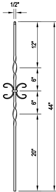
SINGLE BUTTERFLY 1/2" x 44"
