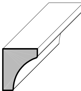
TREAD COVE 5/8" x 3/4"
