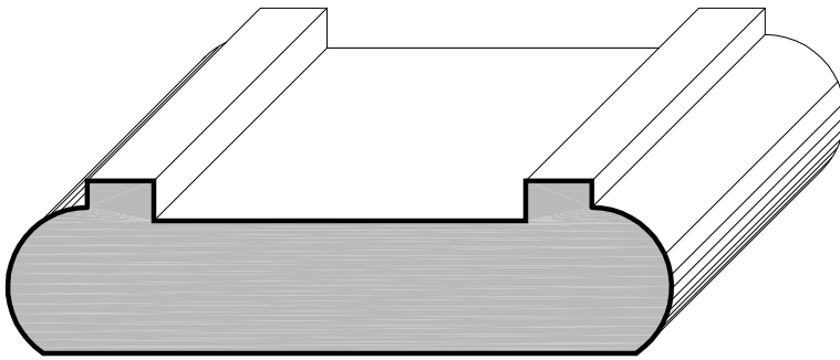
RS01 13/16" x 3 1/8" (SHOWN WITH 3/16" x 1 3/4" PLOW)
