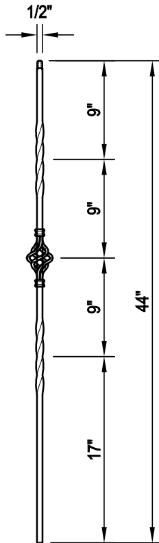
SINGLE BASKET 1/2" x 44"
