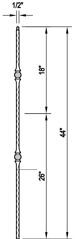
DBL BALL 9/16" x 44"
