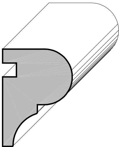
TREAD NOSING 1 1/4" x 1 3/4"
