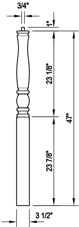
DOWEL TOP 3 1/2" x 47"
