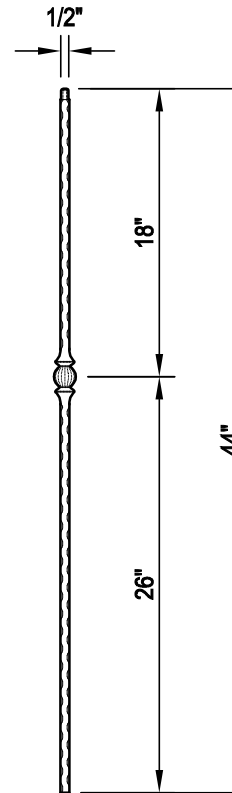
SINGLE BALL 9/16" x 44"
