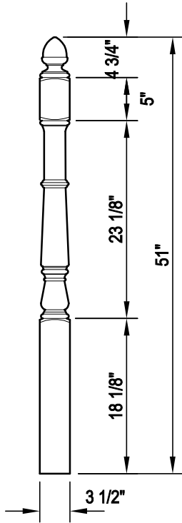
ACORN TOP 3 1/2" x 51"
