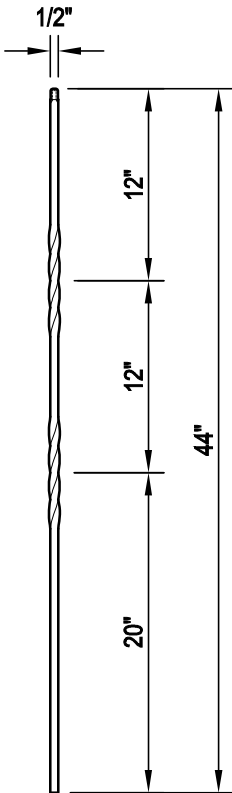
DBL TWIST 1/2" x 44"
