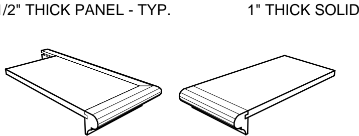
RIGHT HAND TREAD CAP 1 3/4" X 7 1/4" X 12"
