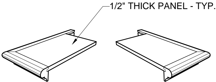
LEFT HAND TREAD CAP 1 3/4" X 7 1/4" X 12"
