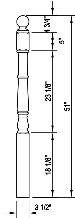
BALL TOP 3 1/2" x 51"
