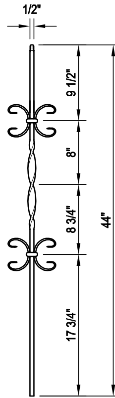
DBL BUTTERFLY 1/2" x 44"
