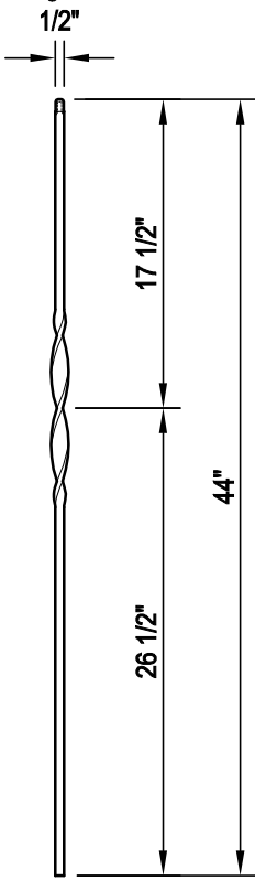
SINGLE RIBBON 1/2" x 44"
